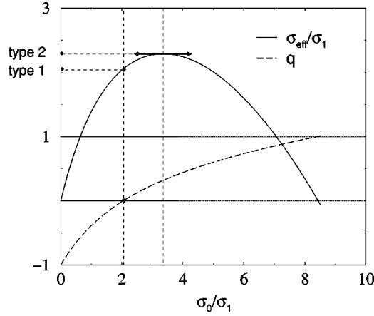
FIG. 6. Rescaled effective conductivity \sigma_{\text{eff}}(\sigma_0)/\sigma_1 , and reduced replica coupling parameter q(\sigma_0) vs \sigma_0 in dimension d=3 for a binary medium. In this example computed from Eqs. (37), (43), the conductivity ratio is \sigma_2/\sigma_1=100 , and the volume fraction p of component 2 is p=0.18 . The “type 1” effective conductivity is obtained when q=0 , whereas the “type 2” effective conductivity corresponds to the maximum of the curve \sigma_{\text{eff}}(\sigma_0) .
