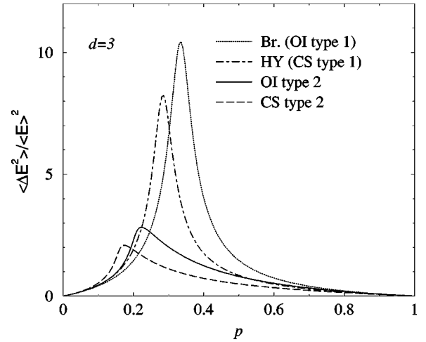
FIG. 5. Relative quadratic fluctuations of the field in dimension d=3 for a binary medium, versus the volume concentration p of component 2. The conductivities are \sigma_1=1, \sigma_2=1000 .
