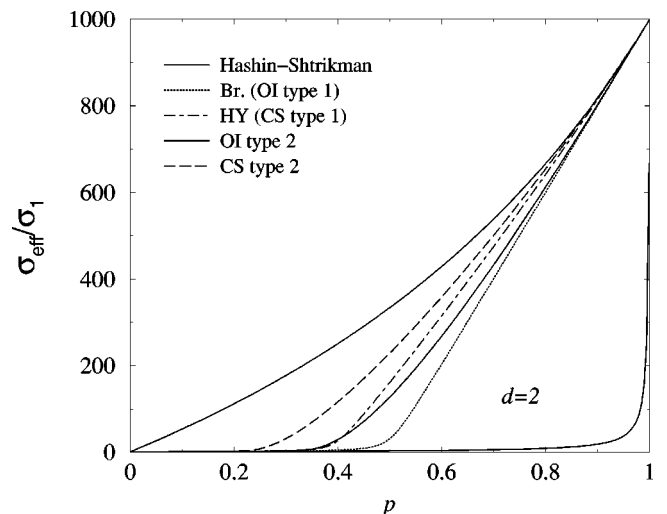
FIG. 2. Rescaled effective conductivities in dimension d = 2 for a binary medium, versus the volume concentration p of component 2. The conductivity ratio is \sigma_2/\sigma_1 = 1000 . Same plots as in Fig. 1.
