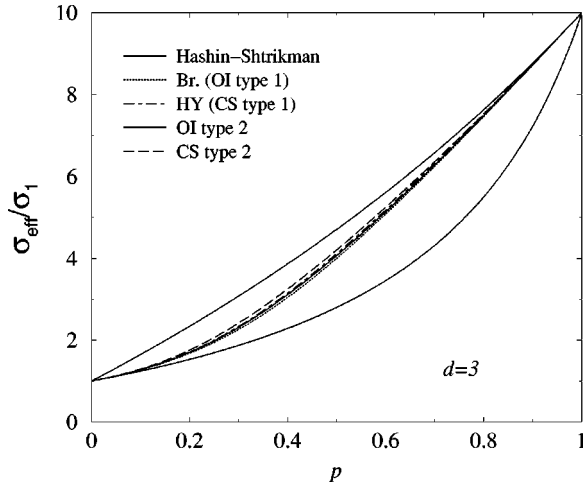
FIG. 3. Rescaled effective conductivities in dimension d=3 for a binary medium, versus the volume concentration p of component 2. The conductivity ratio is \sigma_2/\sigma_1=10 . Same plots as in Fig. 1.
