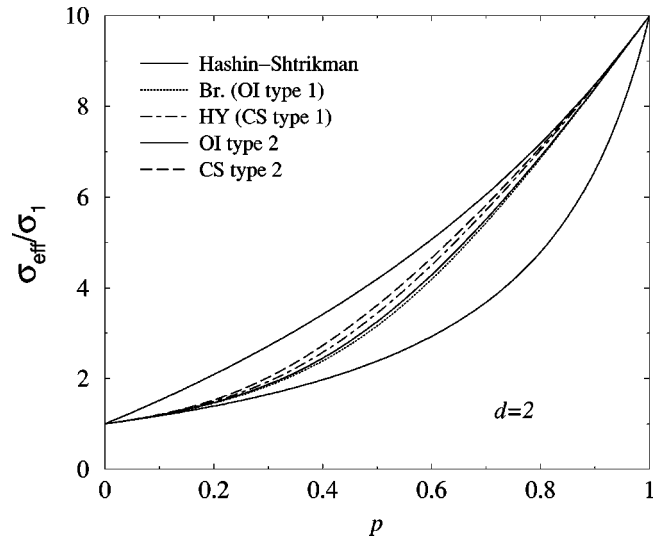
FIG. 1. Rescaled effective conductivities in dimension d = 2 for a binary medium, versus the volume concentration p of component 2. The conductivity ratio is \sigma_2/\sigma_1 = 10 . Highest and lowest solid curves: Hashin-Shtrikman bounds; Br.: the Bruggeman formula (‘‘type 1,’’ one-impurity approximation—OI); HY: the Hori-Yonezawa formula (‘‘type 1,’’ cumulant series approximation—CS); both ‘‘type 2’’ curves are the unique formulas, within OI and CS approximations.
