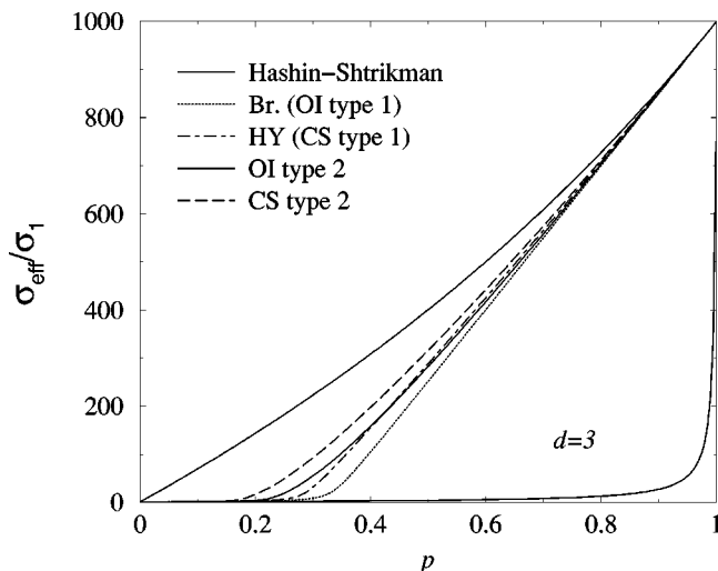
FIG. 4. Rescaled effective conductivities in dimension d=3 for a binary medium, versus the volume concentration p of component 2. The conductivity ratio is \sigma_2/\sigma_1=1000 . Same plots as in Fig. 1.
